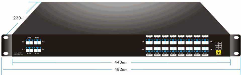
Figure 3 19" Inch 1U Rack
