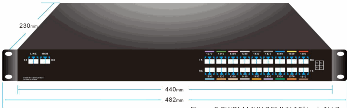
Figure 3 CWDM MUX DEMUX 19" Inch 1U Rack
