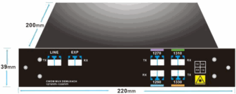
Figure 3 Plug-in LGX Box
